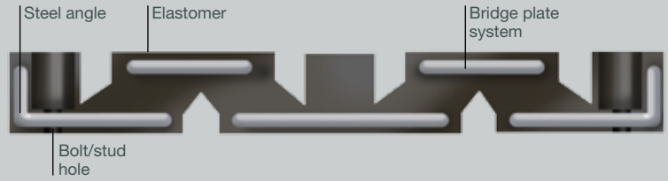
Transflex bridge joint 400, 650, 900 and 1300
