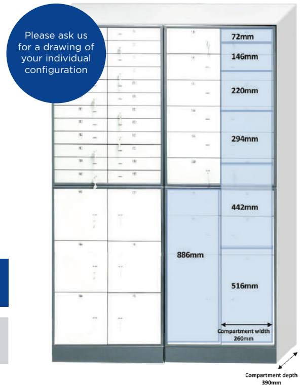
Possible locker unit dimensions
