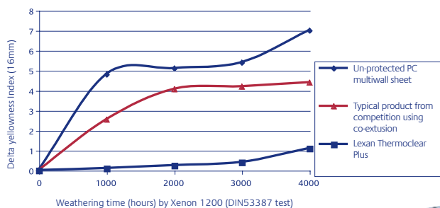
Figure 1 Yellowness index through weathering
